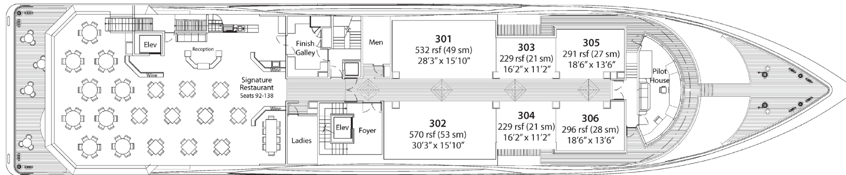
DECK 3
